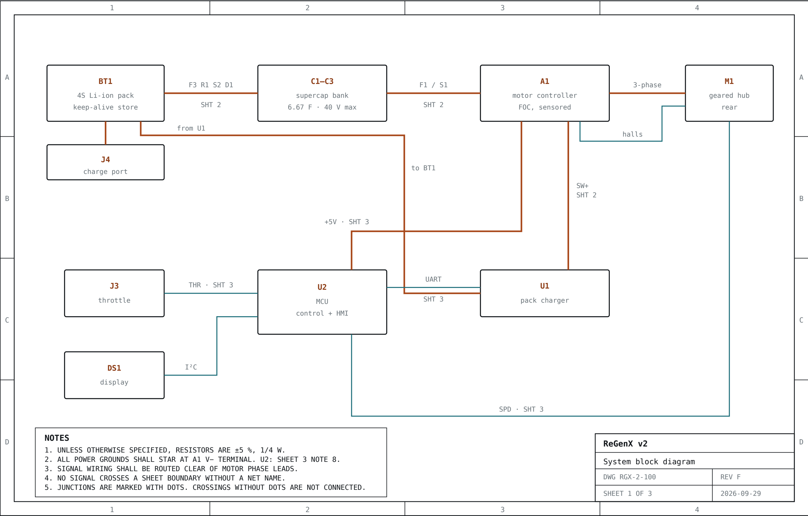
Sheet 1 of 3 – System block diagram
