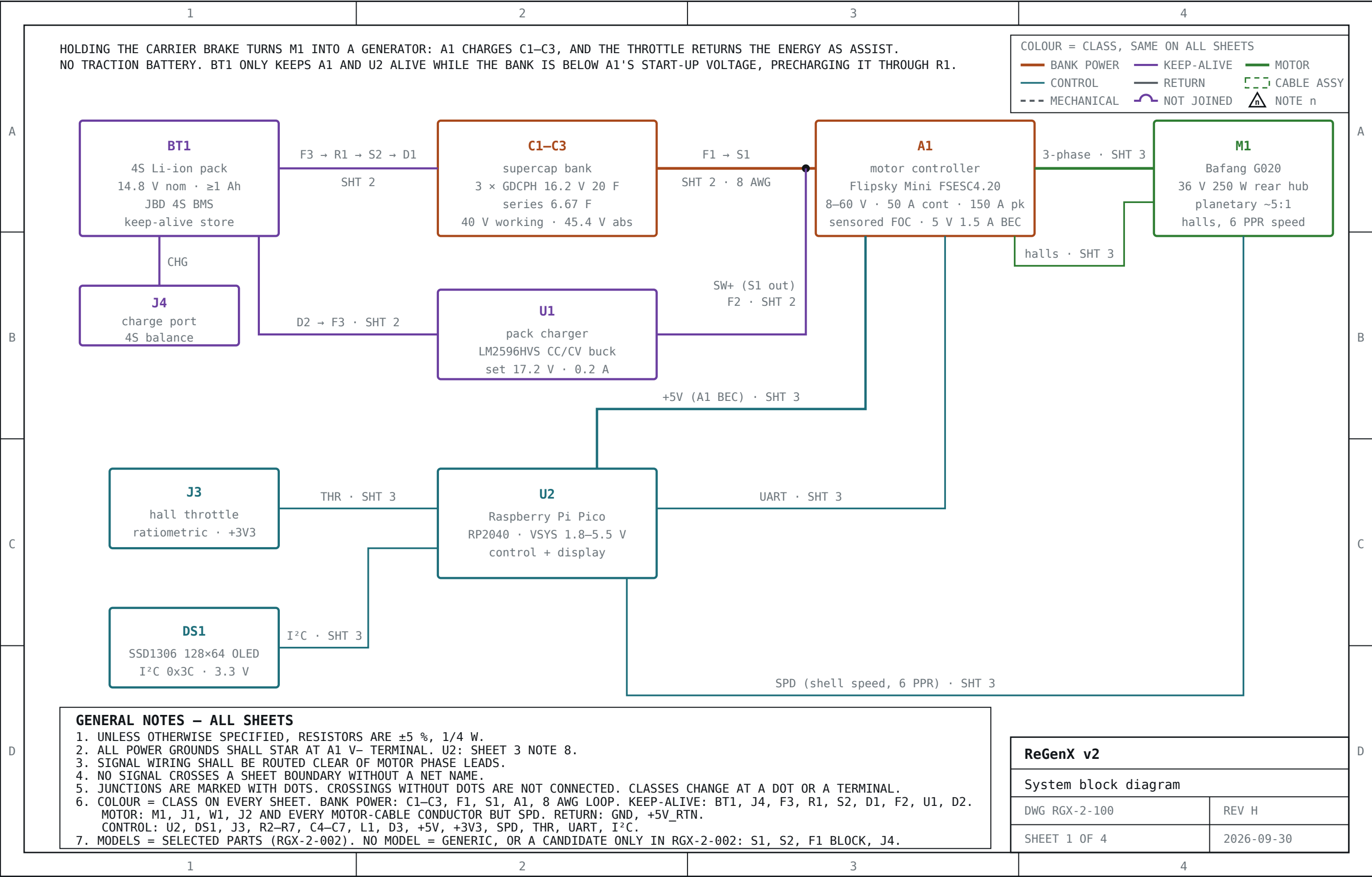
— Sheet 1 of 4 – System block diagram
