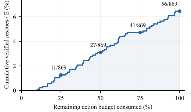
Figure S3. Recovery takes continued action. At 25/50/75/100% of the remaining budget, 11/27/41/56 cases have succeeded, out of 869 eligible pairs. All 813 eligible non-rescues reach their original horizons. The curve describes recorded success timing, not performance under alternative intervention times.
