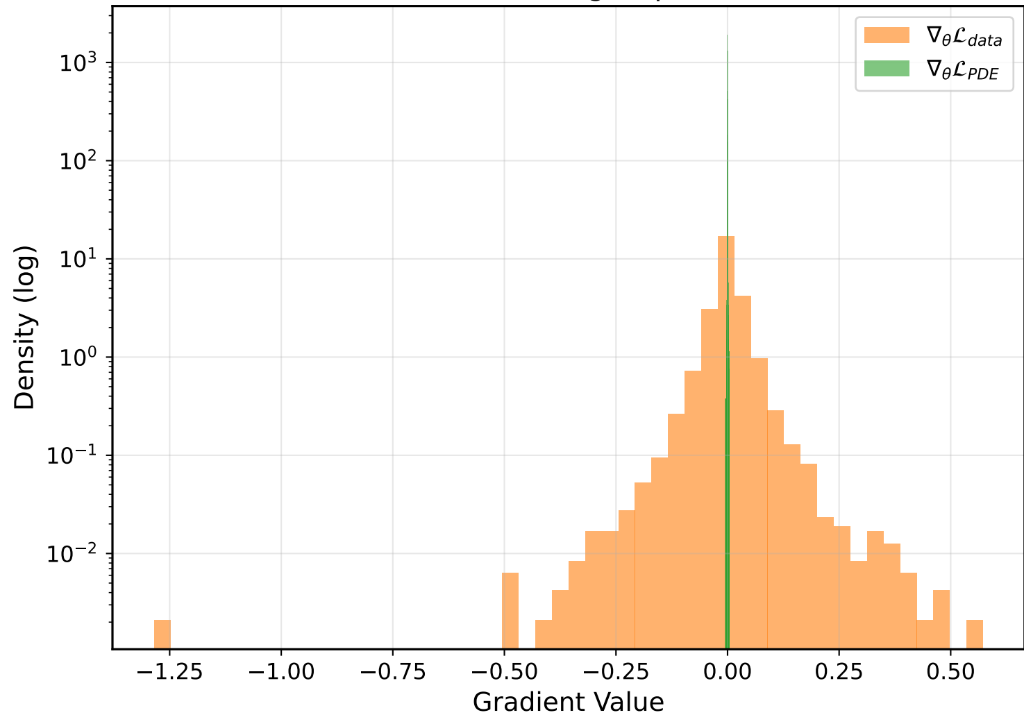
Before Training - Epoch 0
