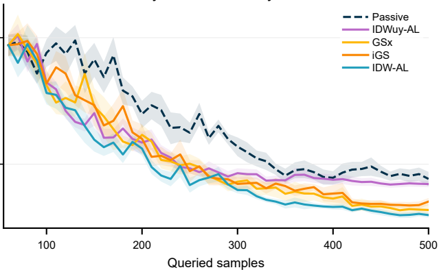
\times 10^{-3} Test RMSE: Ethylene oxidation - with y constraints
