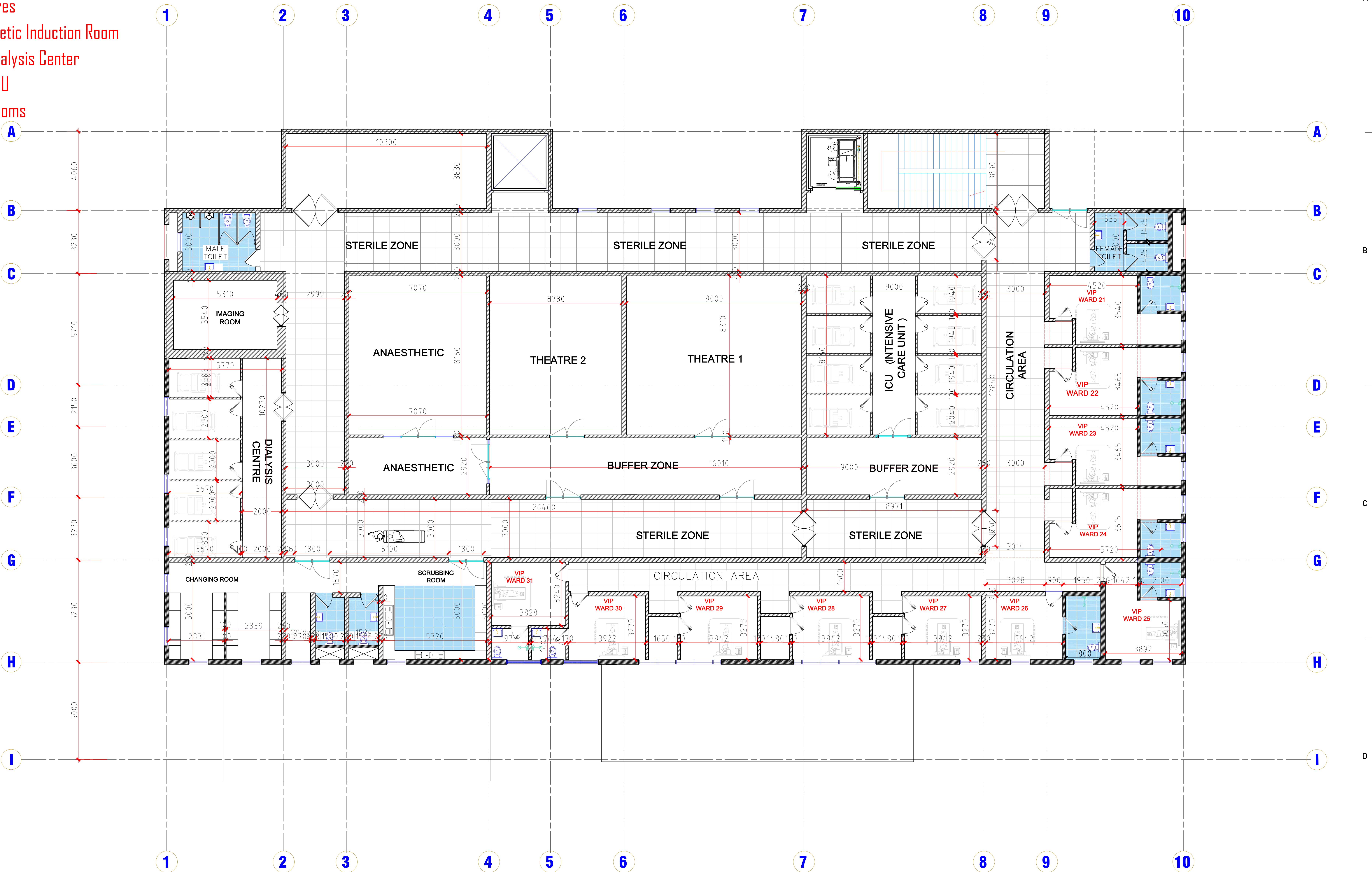
SECOND FLOOR PLAN
