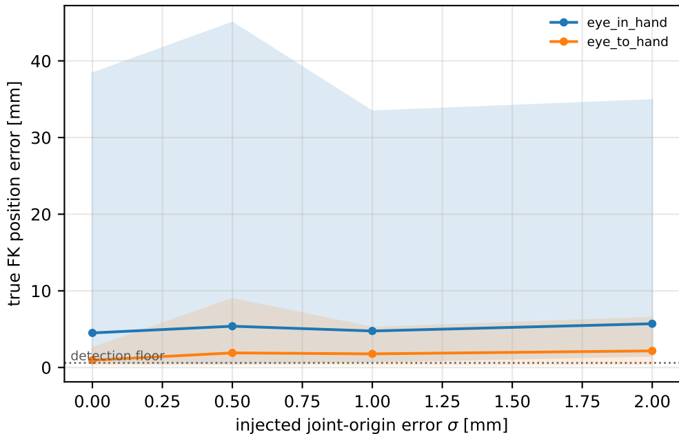
WP4: recovery vs. injected error magnitude
