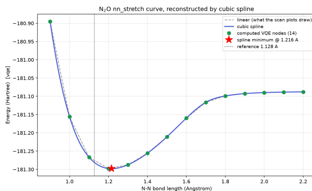
Figure 94: N 2 O N–N stretch, cubic spline reconstruction, RMS 2.526 mHa.
