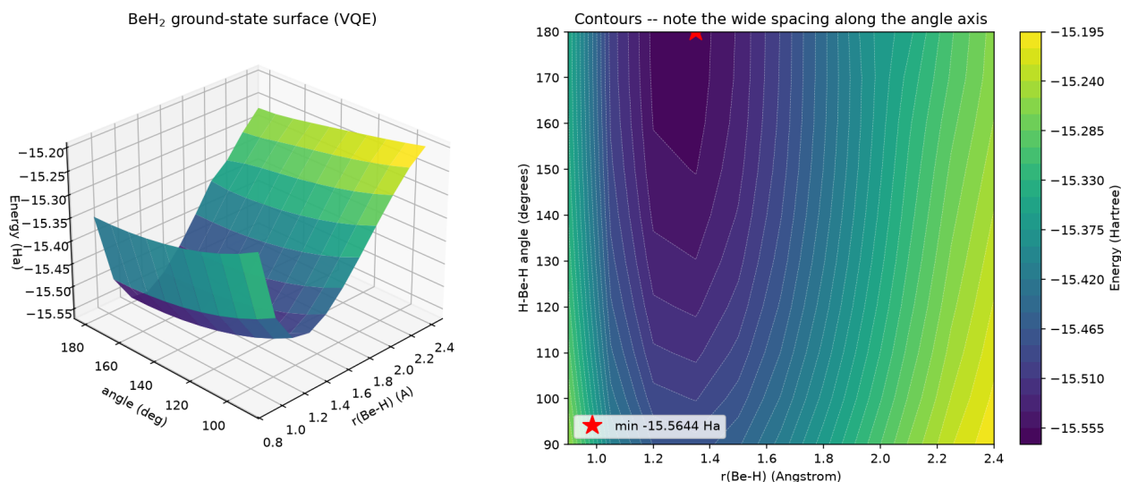
Figure 7: \text{BeH}_2 completed energy surface, static render. The minimum sits at the linear geometry \theta = 180^\circ , as expected for a D_{\infty h} molecule.
