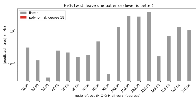
Figure 67: \text{H}_2\text{O}_2 twist, polynomial versus linear leave-one-out error.
