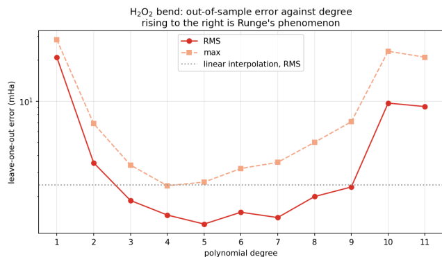
Figure 56: H 2 O 2 bend degree sweep; best degree 5.
