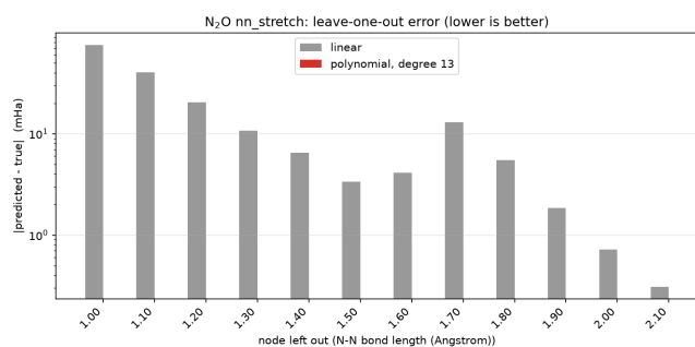
Figure 93: N 2 O N–N stretch, polynomial versus linear leave-one-out error.
