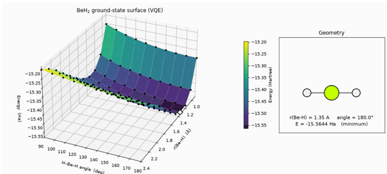
Figure 6: \text{BeH}_2 ground-state energy surface (animation frame). 110 VQE energies rise out of a bond-length \times bond-angle grid in scan order while the molecular rendering redraws to match. The trough runs along the angle axis: bending is soft, stretching is stiff. The reconstruction analysis below turns this into a number.
