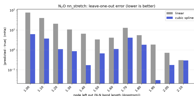
Figure 95: N 2 O N–N stretch, spline leave-one-out error.
