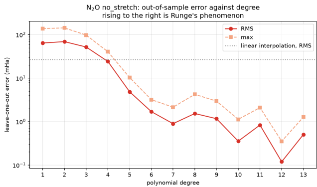
Figure 97: N 2 O N–O stretch degree sweep. Contrast the shape with the N–N sweep (Fig. 92), the same molecule, opposite verdicts.
