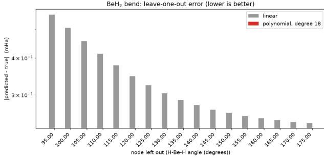
Figure 10: BeH 2 bend, polynomial versus linear leave-one-out error.
