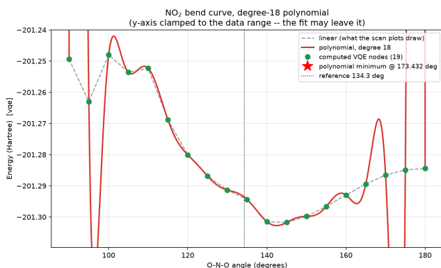
Figure 71: \text{NO}_2 bend, polynomial reconstruction.
