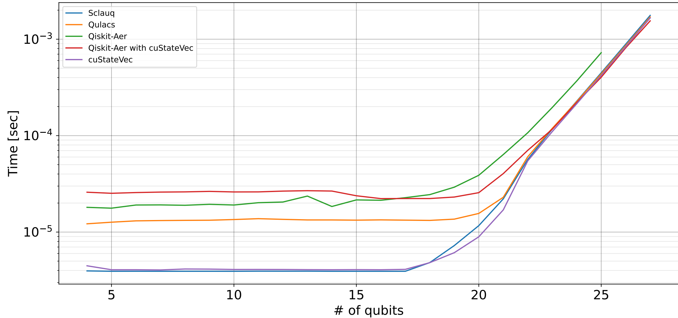
CX Gate apply@Nvidia A100 40 GB
