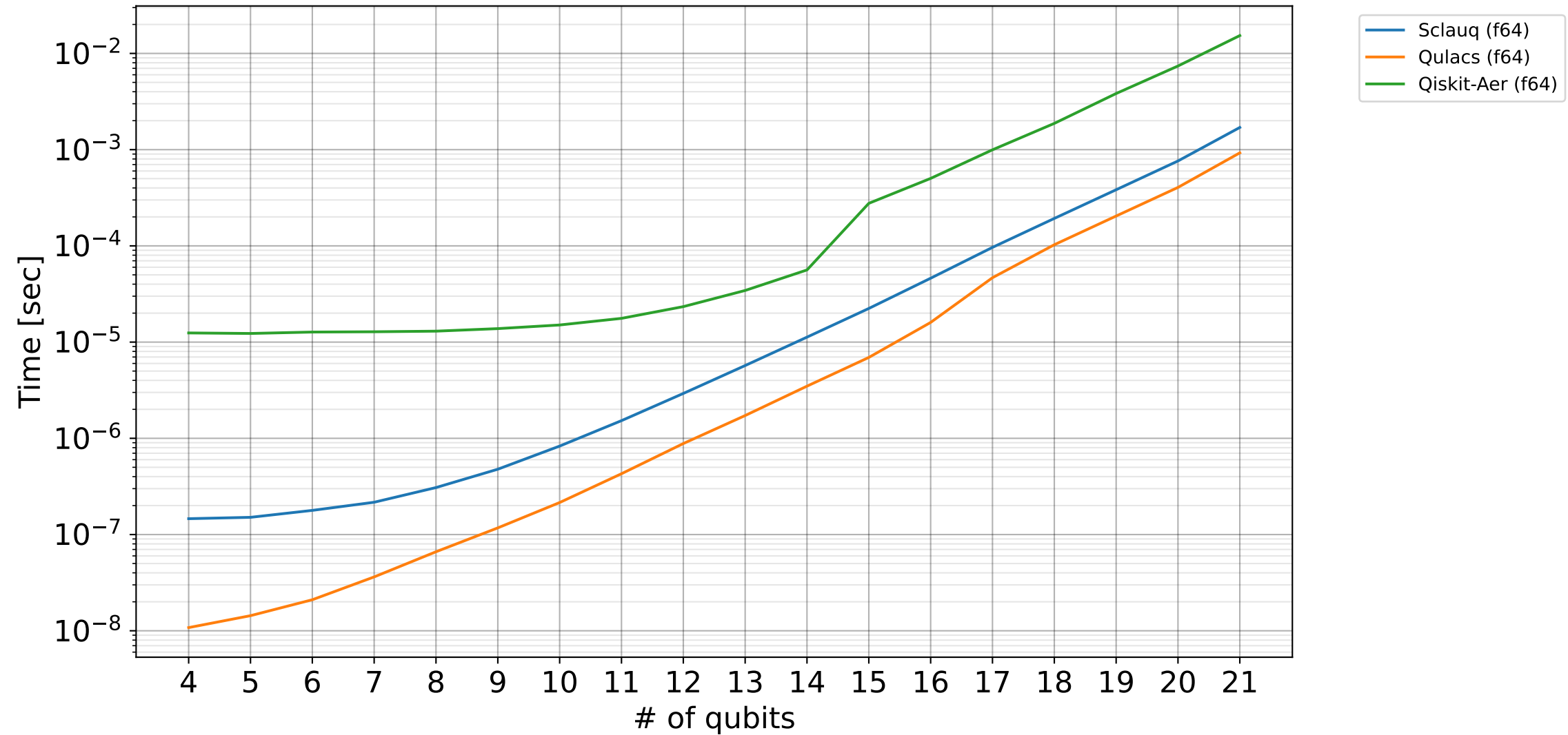
CX Intel(R) Xeon(R) Platinum 9242 CPU @ 2.30GHz singlethread
