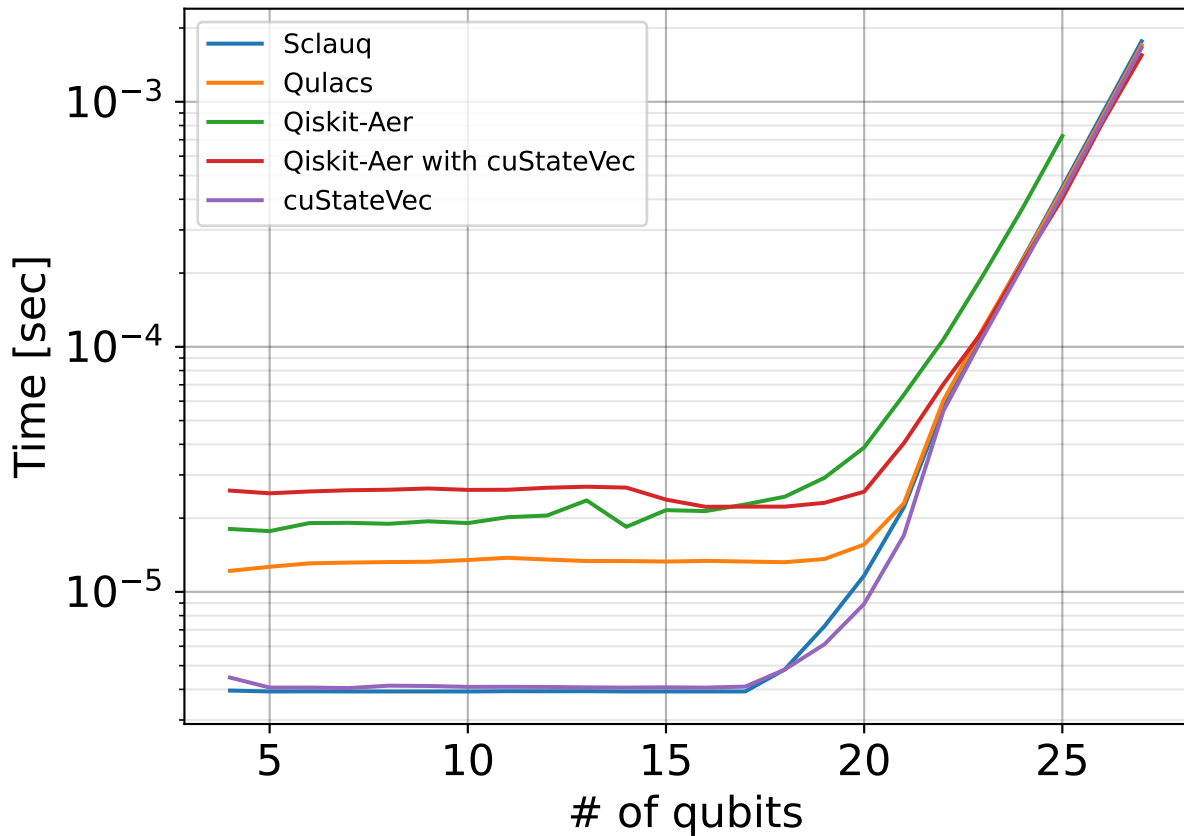
CX Gate apply@Nvidia A100 40 GB
