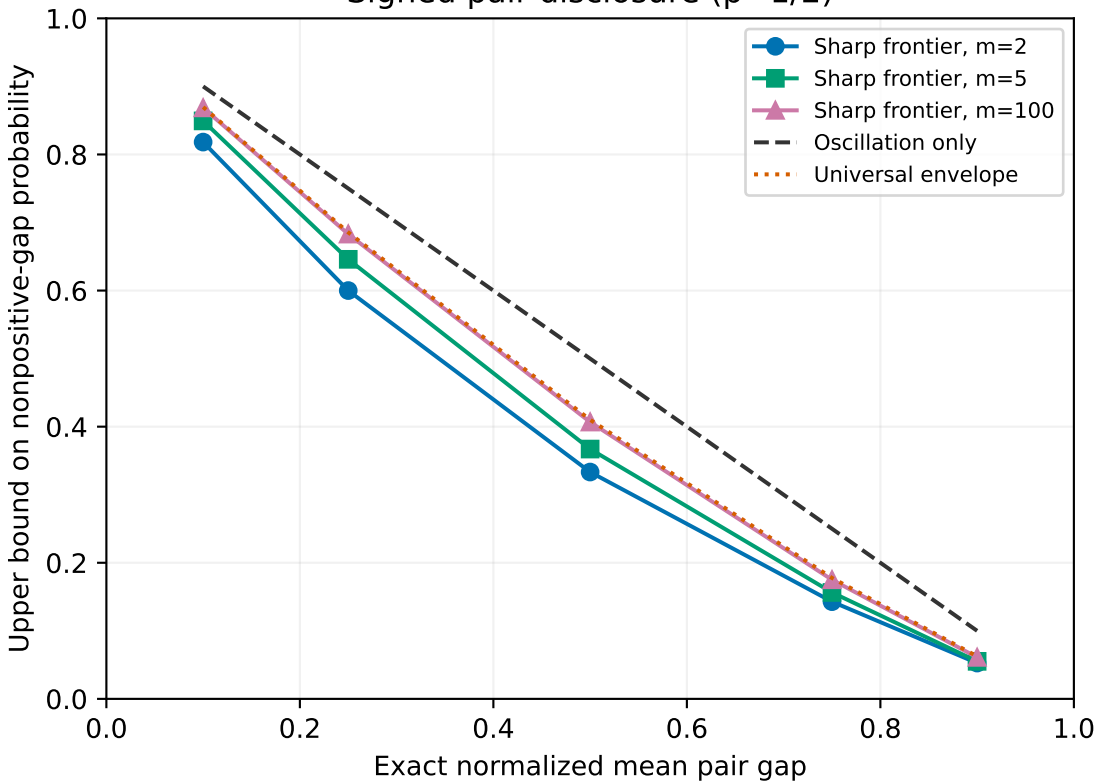
Signed pair disclosure ( p=1/2 )
