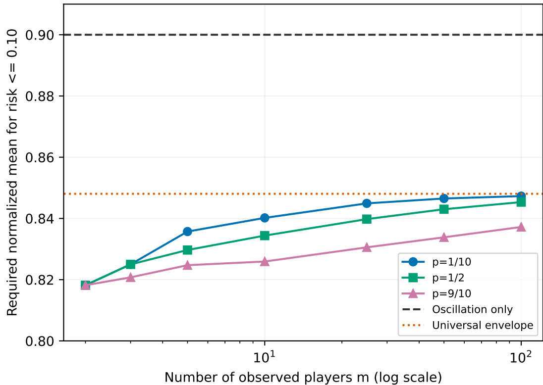
Finite dimensions approach the envelope
