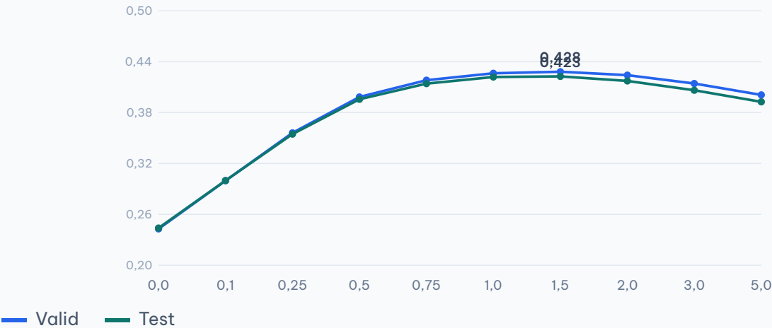
NDCG@5 theo w (w = 0 là plain)
