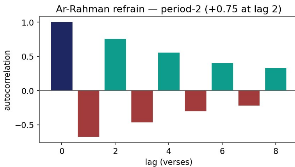
Figure 3. Autocorrelation of Surat ar-Rahman's refrain: a period-2 signature (+0.75 at lag 2).
