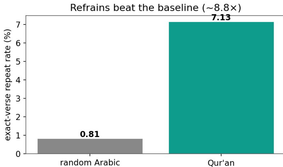
Figure 4. Exact-verse repetition beats the natural-language baseline (7.1% vs 0.81%, \sim 8.8\times ).
