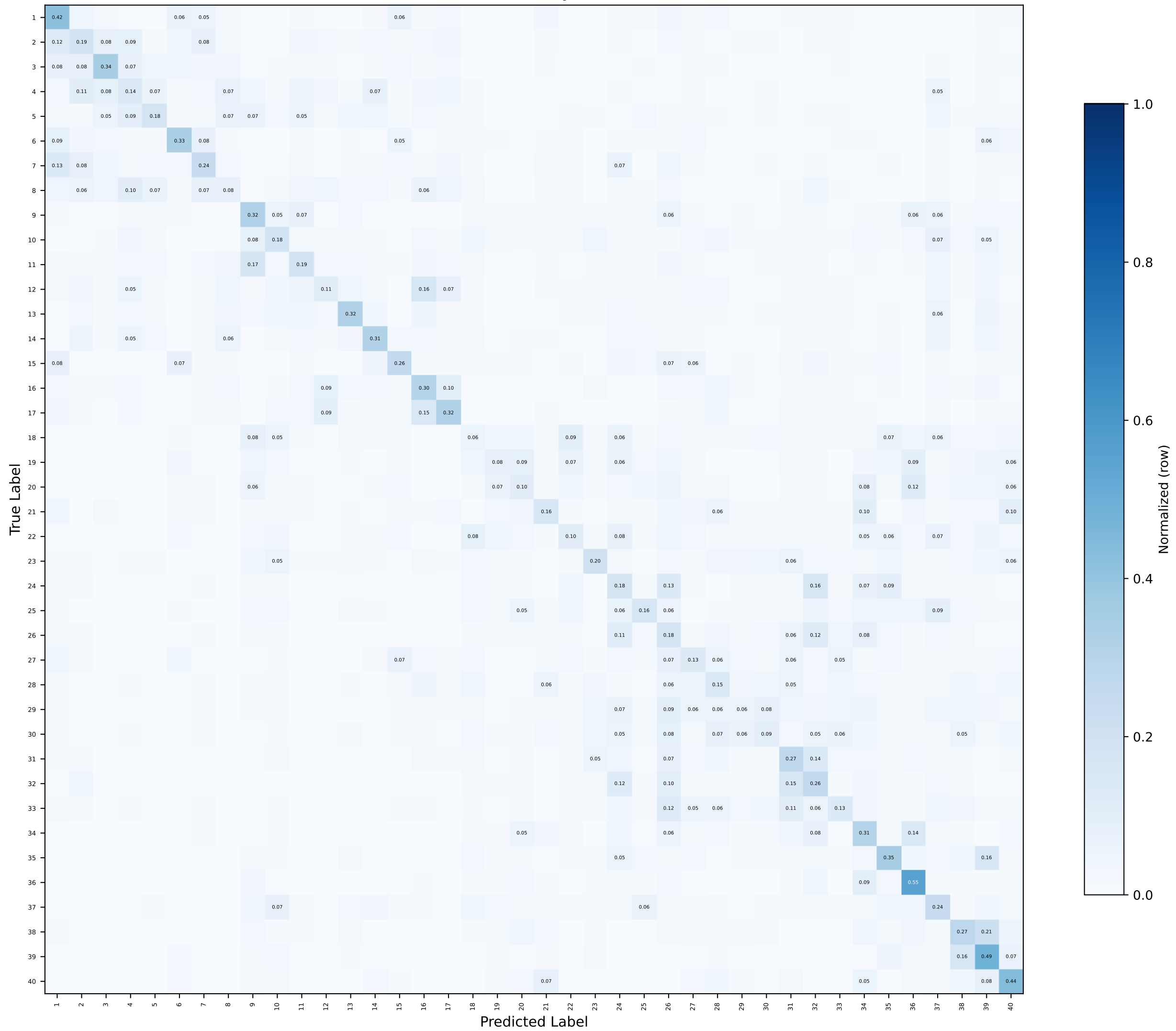
Aggregate Confusion Matrix — DB7 XGBoost LOSO-CV (22 subjects), 40 classes Overall Accuracy: 23.1%
