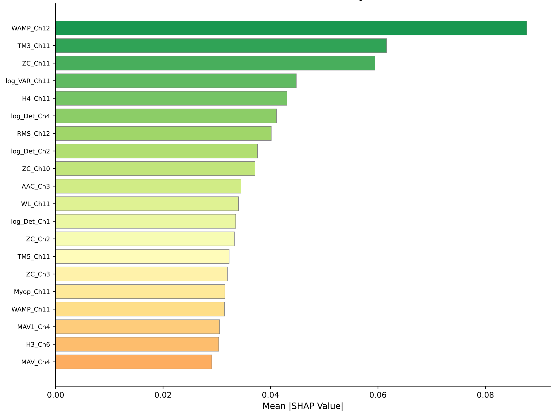
Top 20 SHAP Feature Importance — DB2 (LOSO-CV, XGBoost, 40 subjects)
