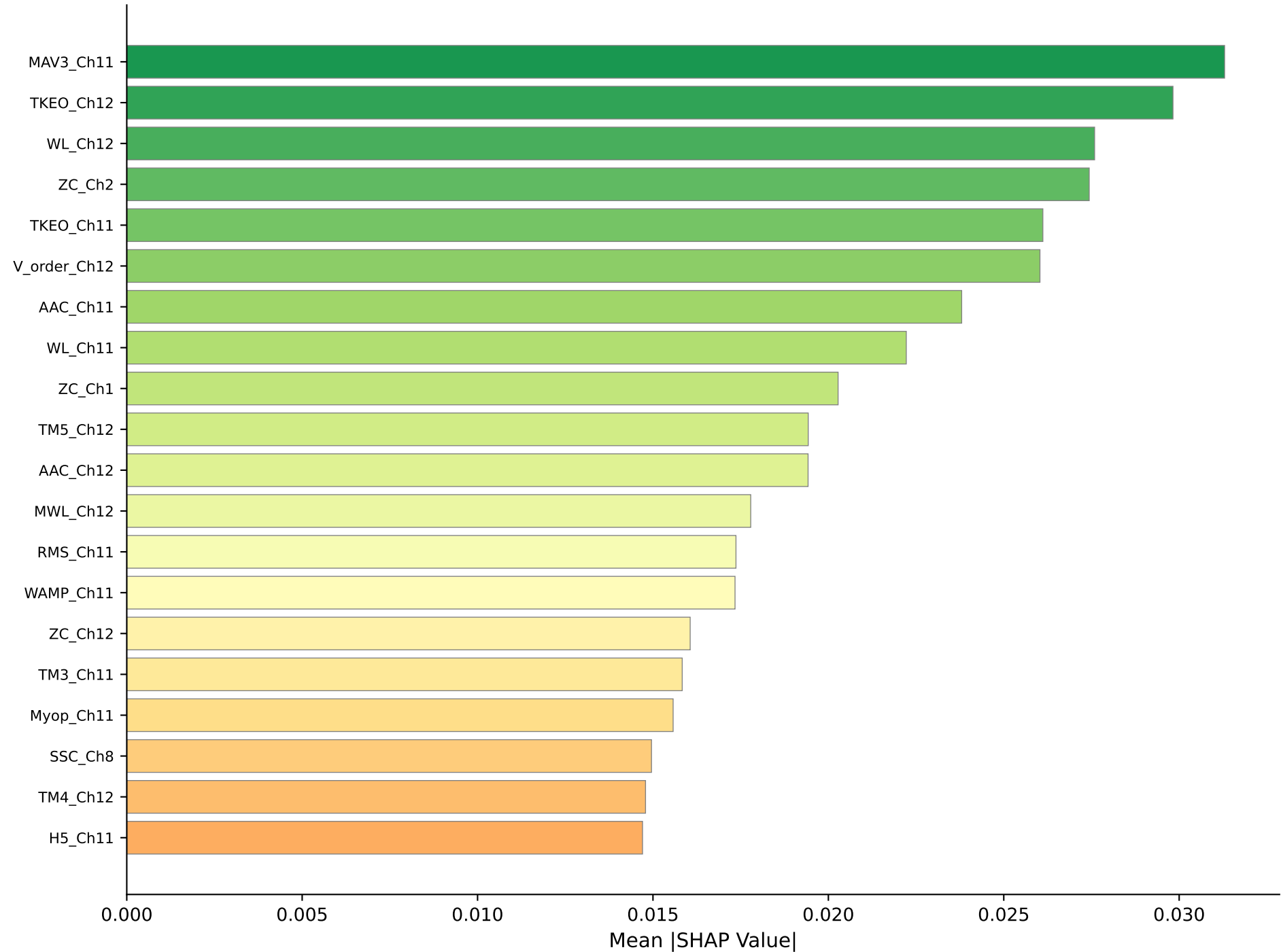
Top 20 SHAP Feature Importance — DB3 (LOSO-CV, XGBoost, 11 subjects)
