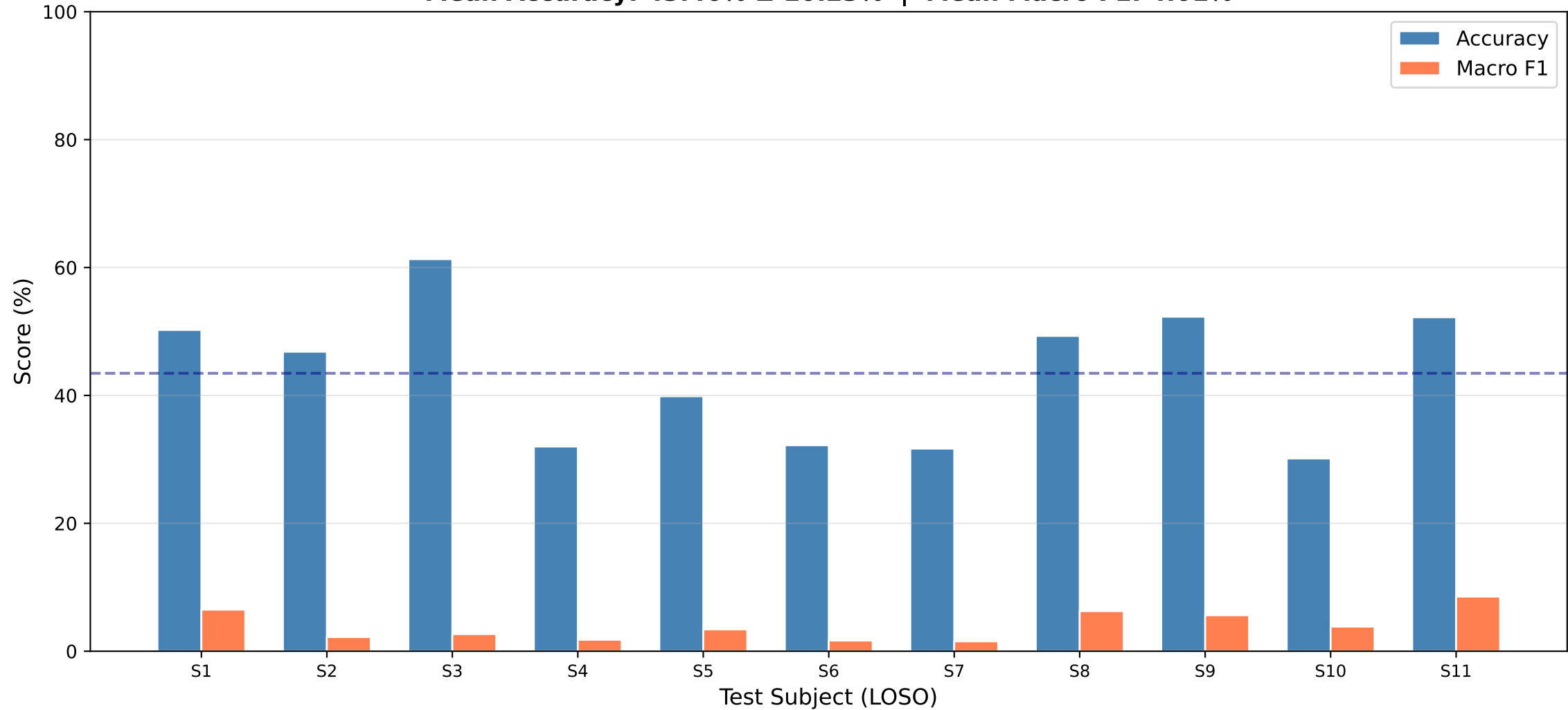
Per-Subject Performance — XGBoost on NinaPro DB3 Mean Accuracy: 43.46% \pm 10.23% | Mean Macro F1: 4.01%
