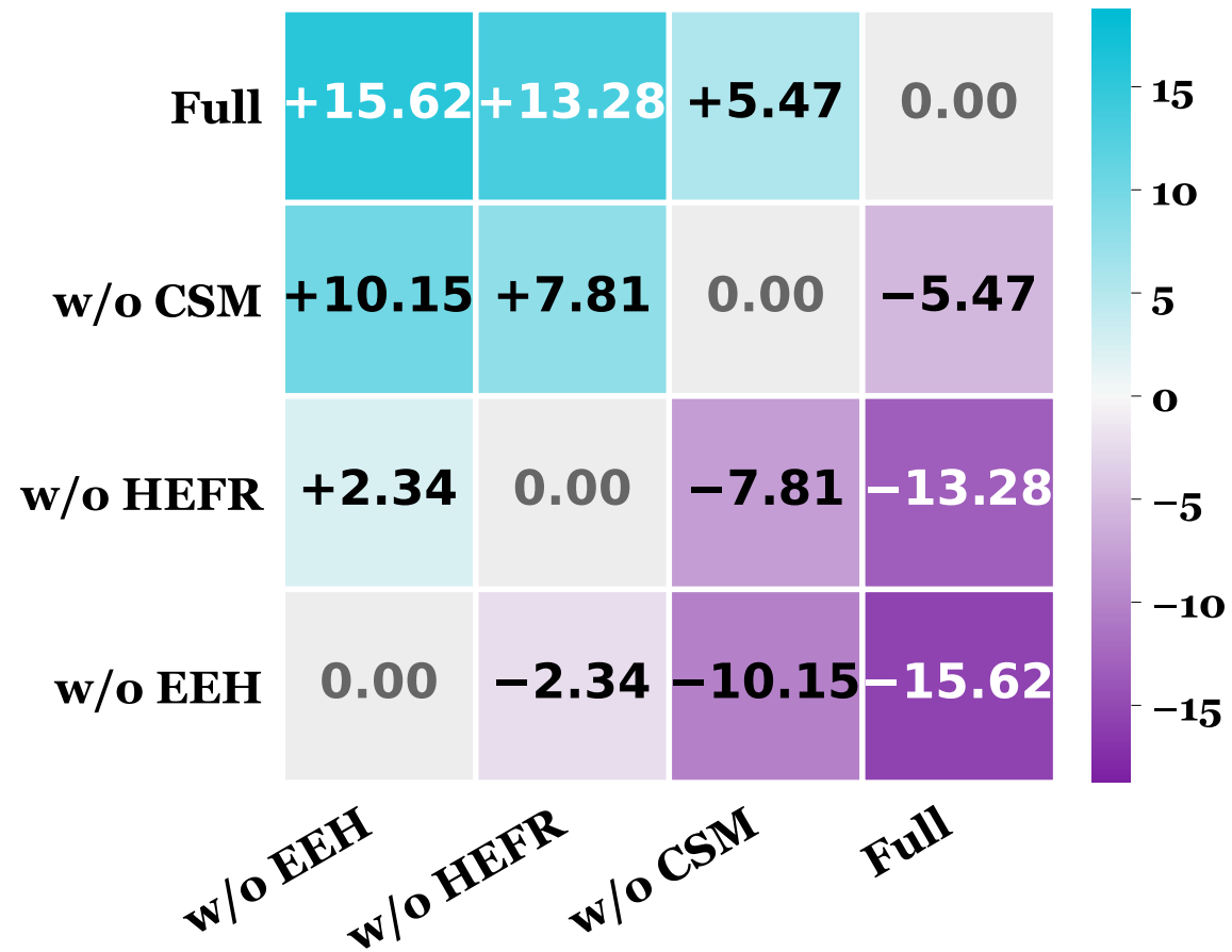
DeepSeek-V4-Flash -- Acc (%)
