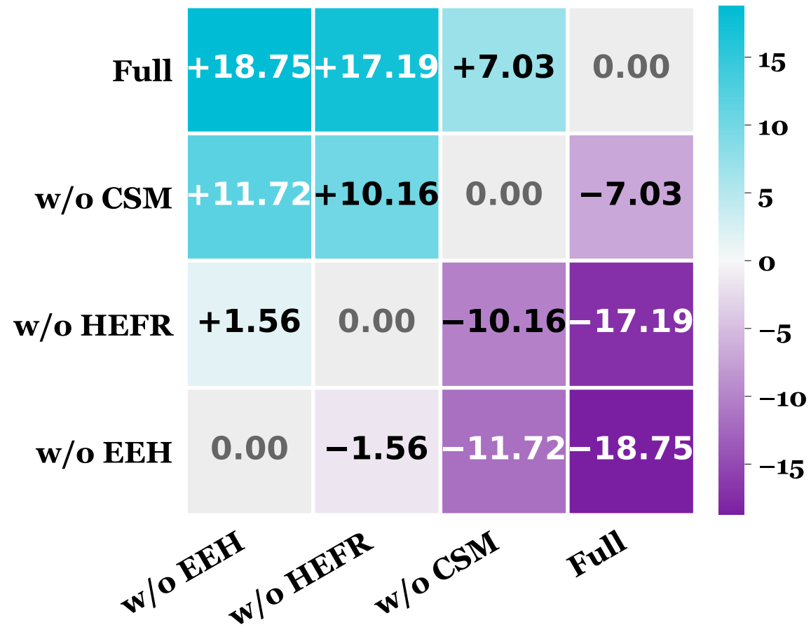
GPT-5.4-mini -- Acc (%)
