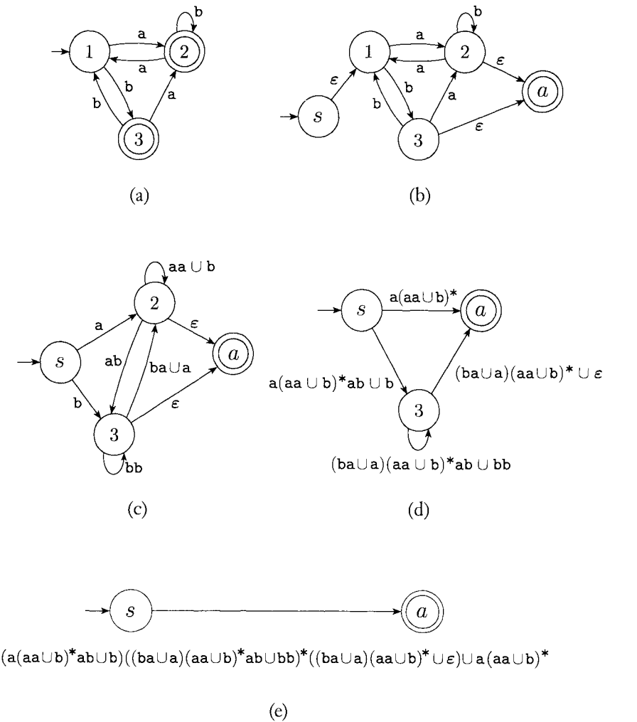
FIGURE 1.69 Converting a three-state DFA to an equivalent regular expression
