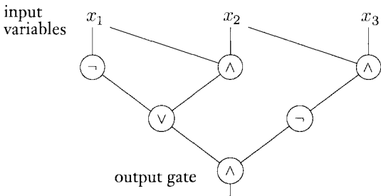
FIGURE 9.23 An example of a Boolean circuit
