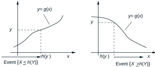
Figure 3.23: Calculating the probability \mathbf{P}(g(X) \leq y) . When g is monotonically increasing (left figure), the event \{g(X) \leq y\} is the same as the event \{X \leq h(y)\} . When g is monotonically decreasing (right figure), the event \{g(X) \leq y\} is the same as the event \{X \geq h(y)\} .
