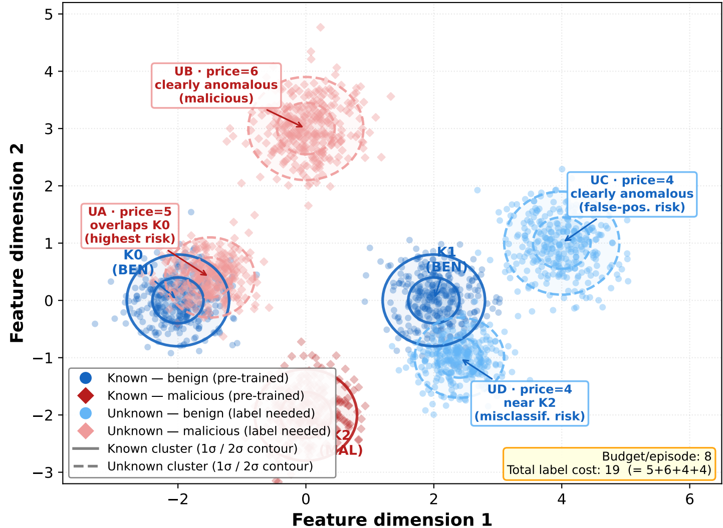
Synthetic LION — Traffic Cluster Feature Space
