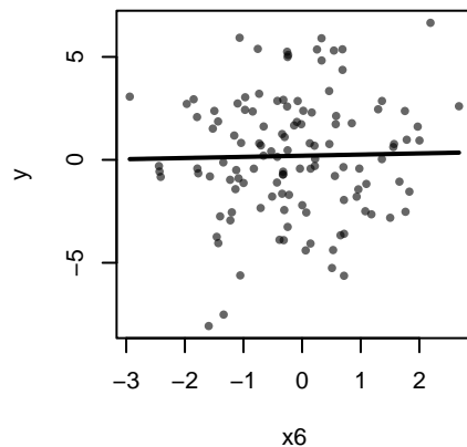
Marginal fit for x6
