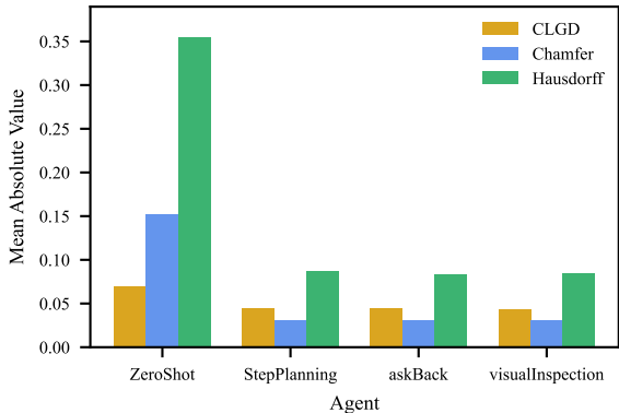
box – Distance Metrics (mean, ChatGPT 4o)
