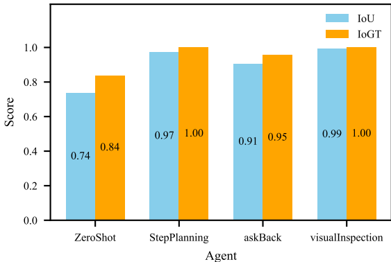
u-profile – IoU and IoGT (ChatGPT 4o)
