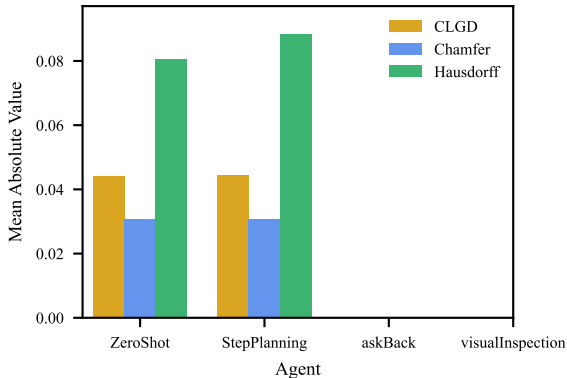
box – Distance Metrics (mean, Claude Opus 4)
