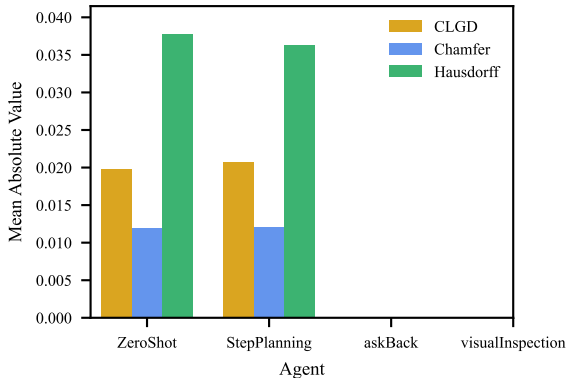
u-profile – Distance Metrics (mean, Claude Opus 4)
