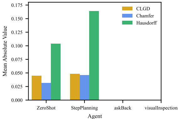
box – Distance Metrics (mean, DeepSeek Chat)
