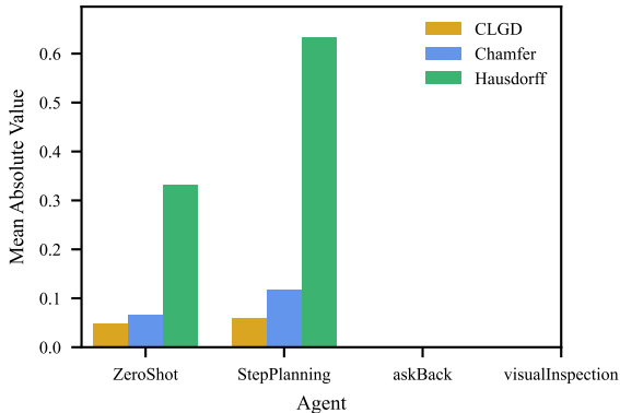
right-angle – Distance Metrics (mean, DeepSeek Chat)
