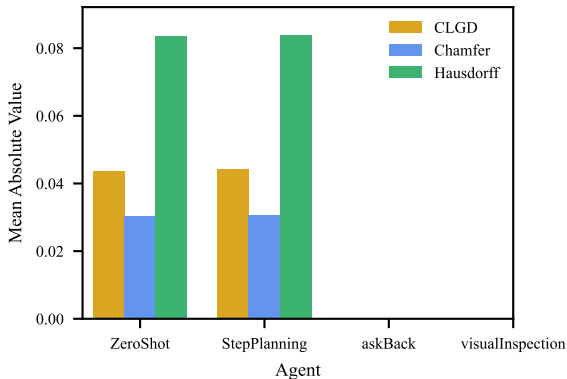
box – Distance Metrics (mean, Gemini 2.5 Pro)
