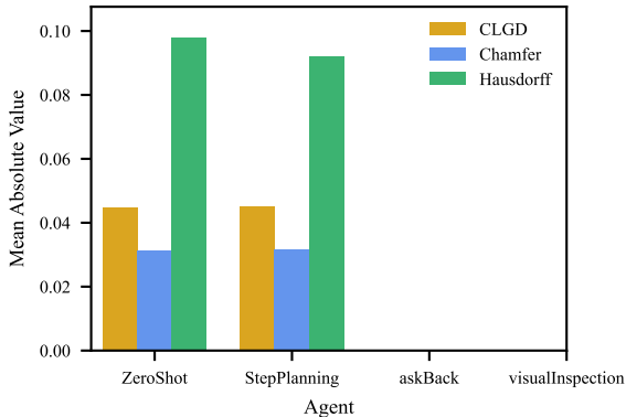
right-angle – Distance Metrics (mean, Gemini 2.5 Pro)
