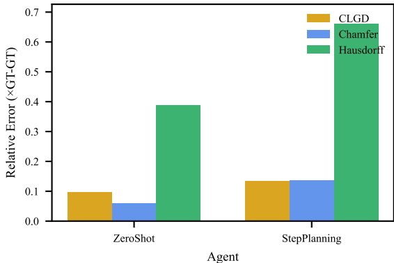
toy-car – Relative Error (Gemini 2.5 Pro)
