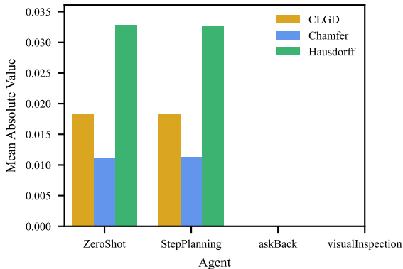
u-profile – Distance Metrics (mean, Gemini 2.5 Pro)
