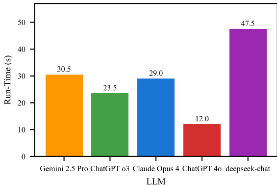
Run-Time mean of zeroShot + stepPlanning by LLM
