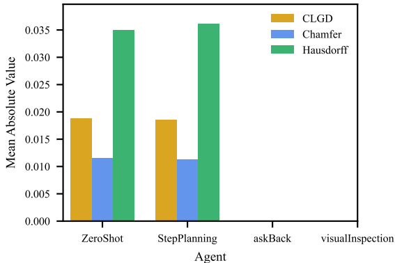
u-profile – Distance Metrics (mean, ChatGPT o3)
