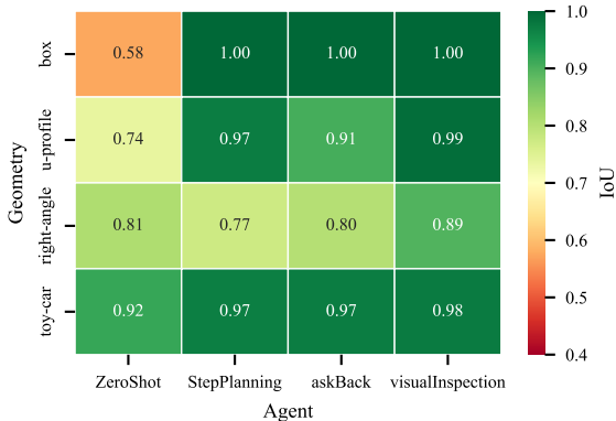
IoU Heatmap by Agent and Geometry (ChatGPT 4o)
