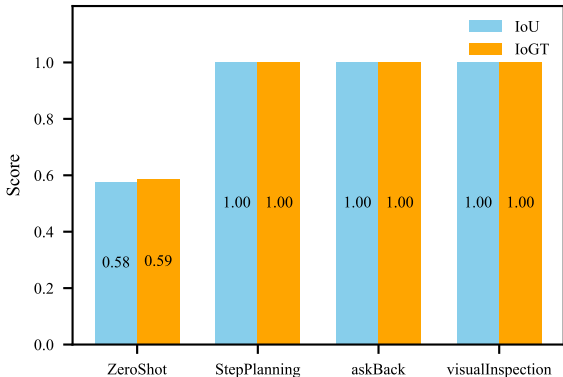
box – IoU and IoGT (ChatGPT 4o)
