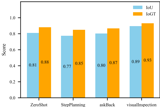
right-angle – IoU and IoGT (ChatGPT 4o)
