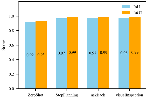
toy-car – IoU and IoGT (ChatGPT 4o)
