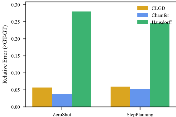
toy-car – Relative Error (Claude Opus 4)
