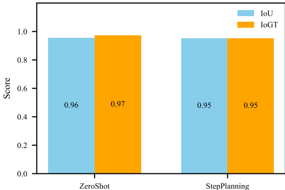
u-profile – IoU and IoGT (Claude Opus 4)
