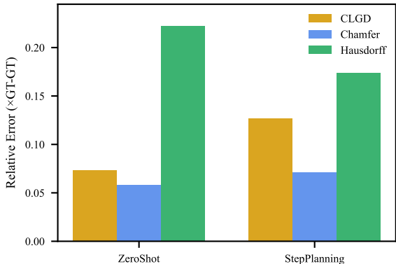
u-profile – Relative Error (Claude Opus 4)
