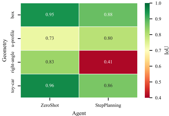
IoU Heatmap by Agent and Geometry (Deepseek Chat)
