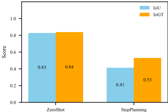
right-angle – IoU and IoGT (Deepseek chat)
