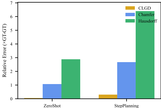
right-angle – Relative Error (Deepseek Chat)
