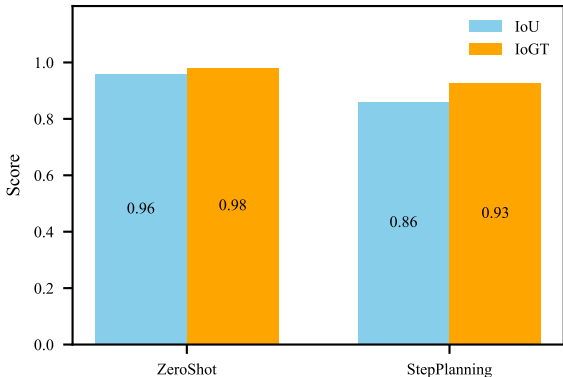
toy-car – IoU and IoGT (Deepseek chat)
