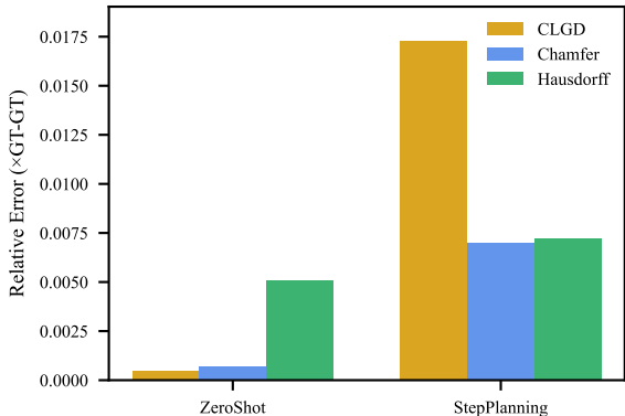
box – Relative Error (Gemini 2.5 Pro)
