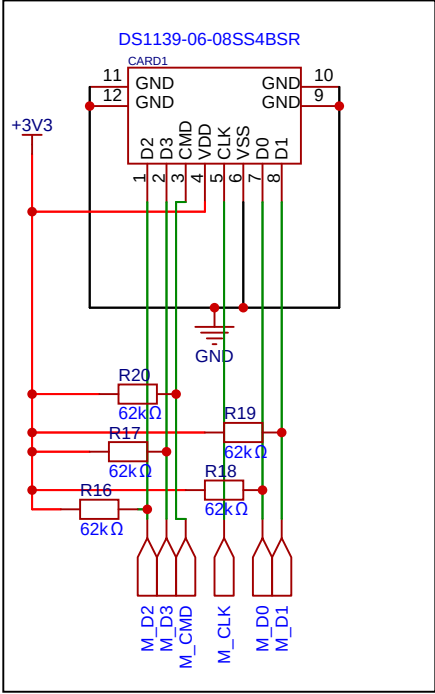
micro-sd card
