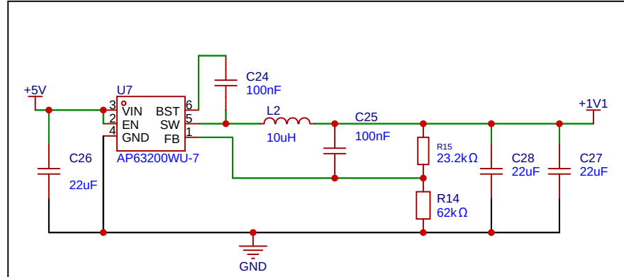
5v -> 1v1
