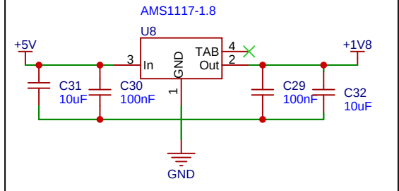
5v -> 1v8
