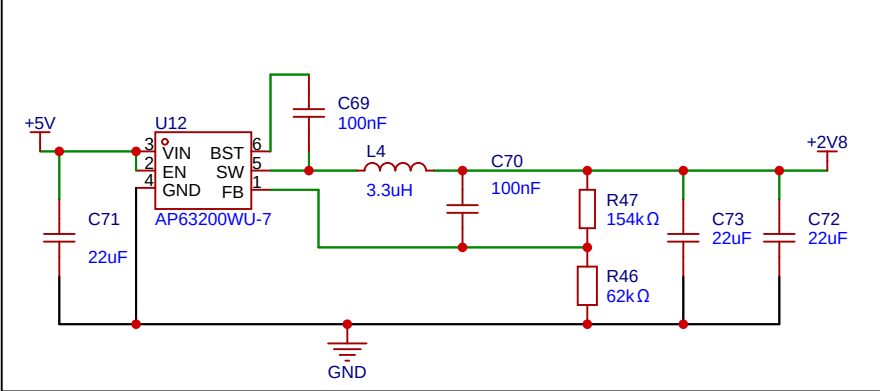
5v -> 2v8
