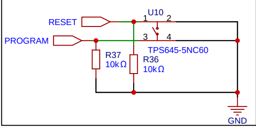
USB-C PROGRAM
