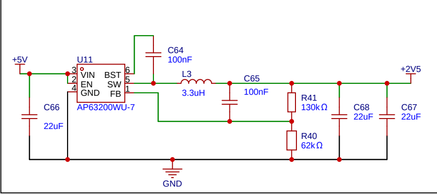
5v -> 2v5
