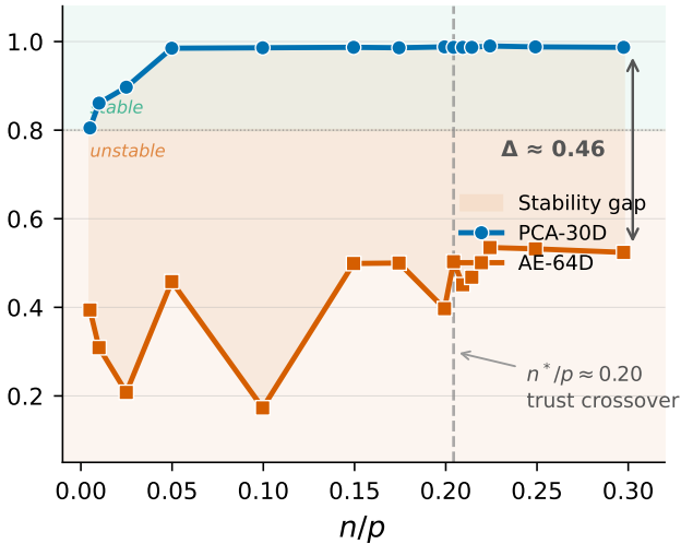
Inter-seed kNN Edge Jaccard
