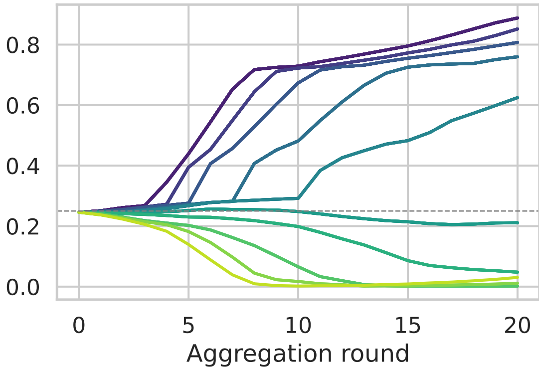
Held-out accuracy
